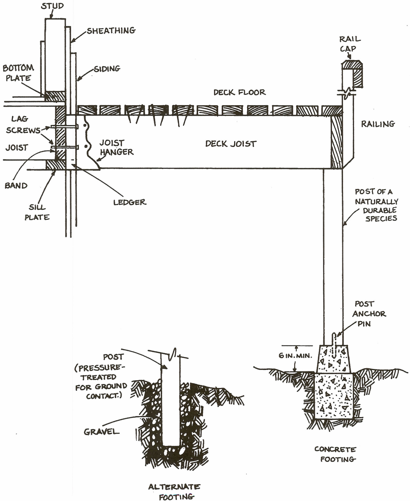
Figure 67. Wood Deck
